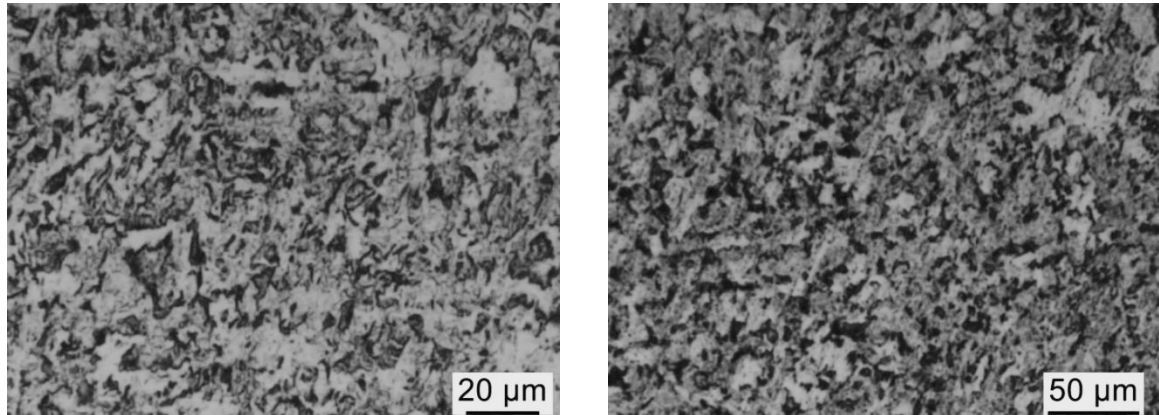
Figure 4. HAZ micro-structure in region of intensive grain growth towards the fusion line
