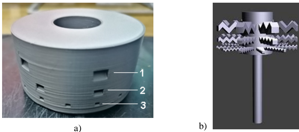
Figure 3: a) Manufactured second prototype by 3D printing using plastics and b) trim space filled with fluid – geometry prepared for CFD
