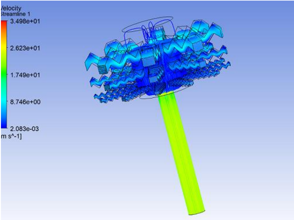
Figure 13: Velocity distribution for the second trim design
