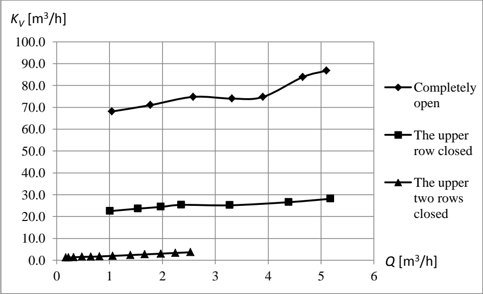
Figure 8: Dependence of the flow coefficient K_V of the volume flow rate Q
