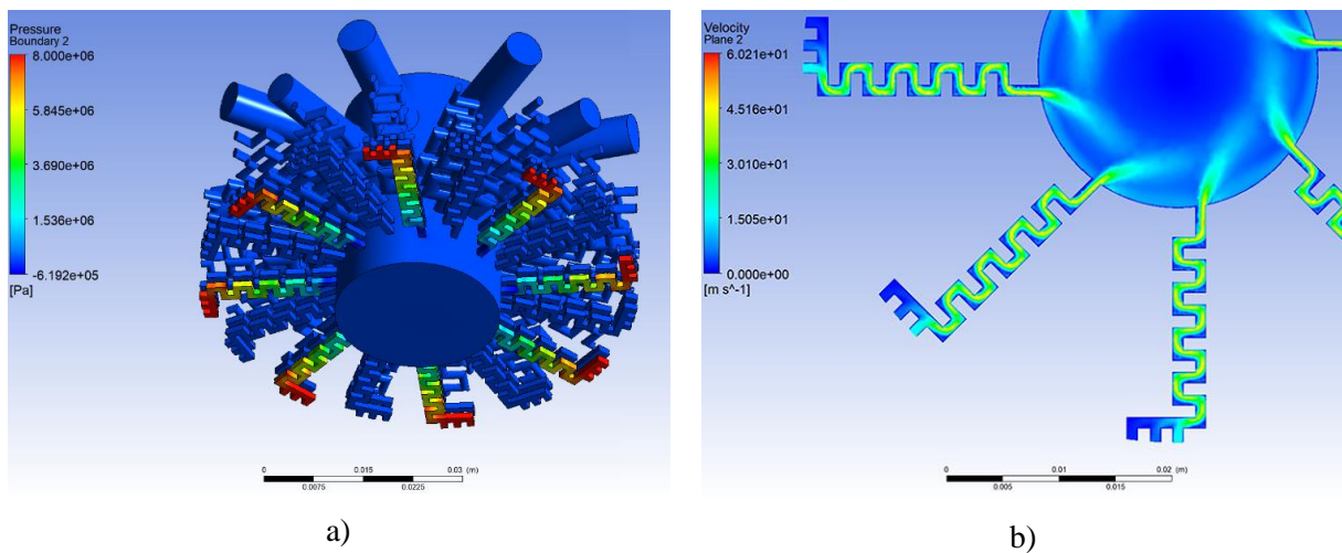
Figure 10: The first trim design for the lowest flow rate a) pressure distribution b) velocity distribution
