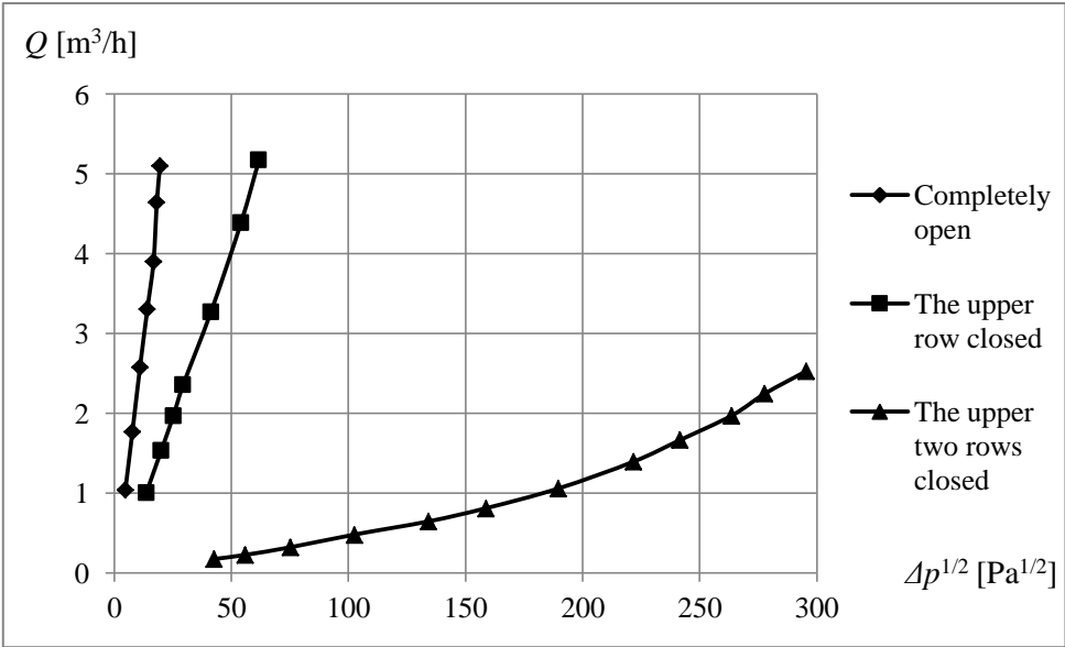
Figure 7: Dependence of the volume flow rate Q of the pressure drop \Delta p
