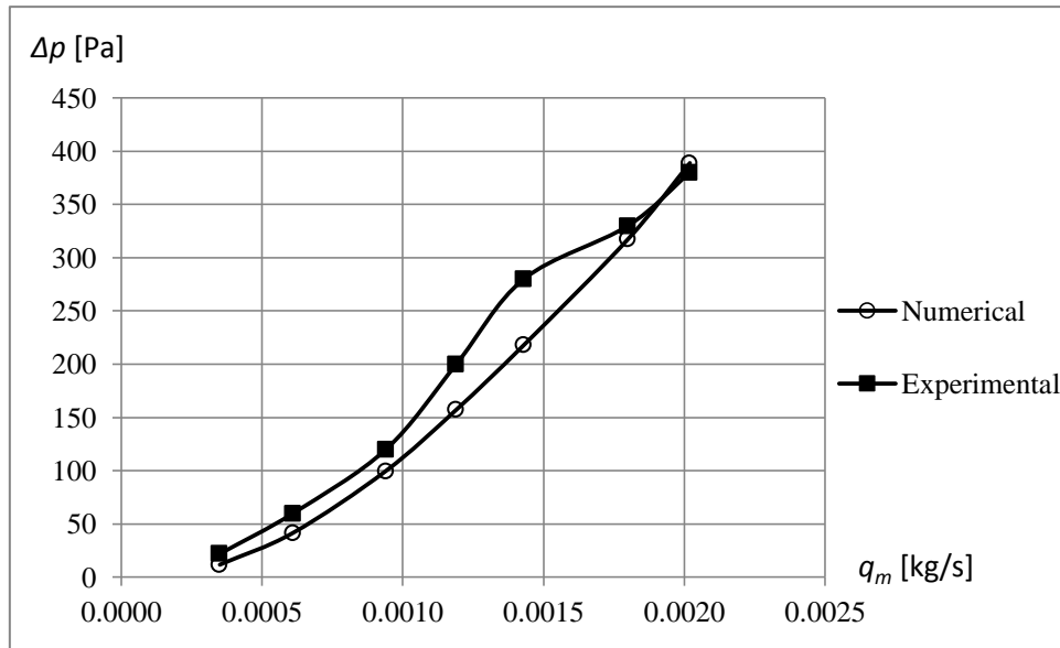
Figure 14: Static pressure drop distribution for the second trim design
