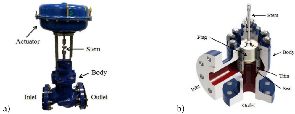
Figure 1: Components of the control valve a) valve with the actuator and b) valve body with the trim [1]
