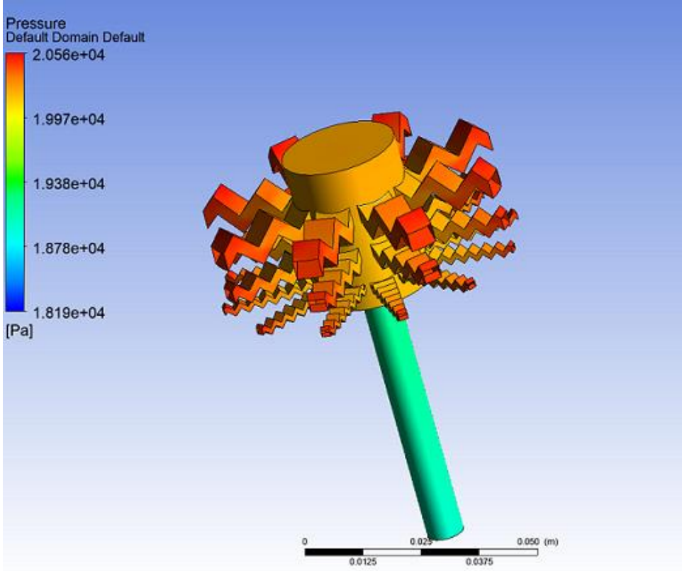
Figure 14: Pressure distribution for the second trim design
