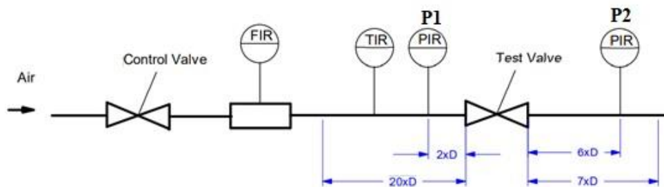
Figure 5: Air test section for the determination of K_V values of test valves according to [6]
