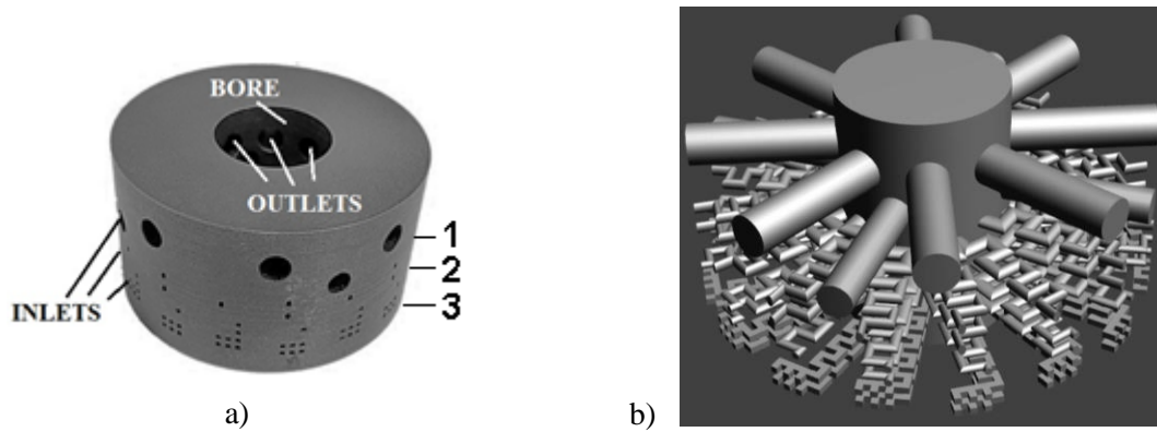
Figure 2: a) Manufactured first prototype by the SLM (selective laser melting) 3D Metal Printing process and b) trim space filled with fluid – geometry prepared for CFD
