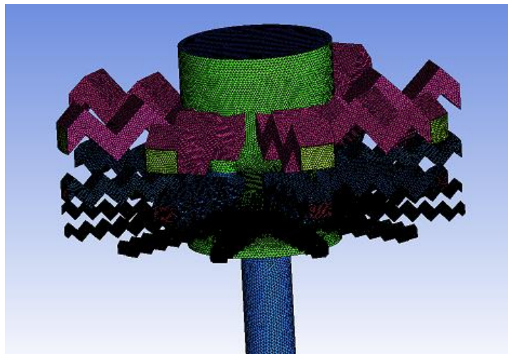
Figure 12: Unstructured mesh for CFD calculations on the second trim design
