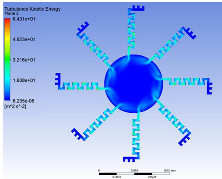
Figure 11: Turbulence kinetic energy for the first trim design
