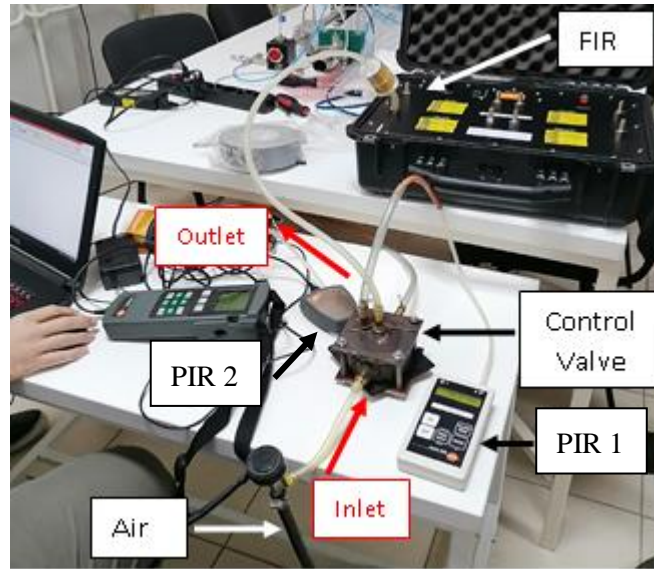
Figure 6: Air test section in laboratory
