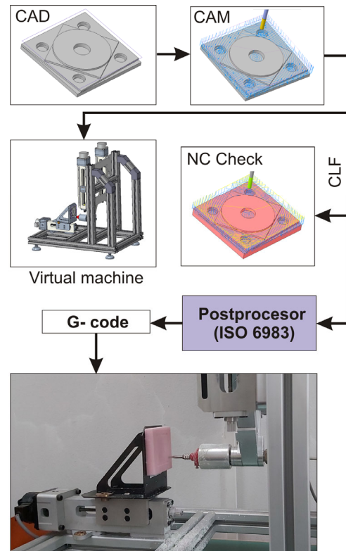
Machining of the workpiece on the machine Fig. 2. Programming method based on CAD/CAM system (PTC Creo)
