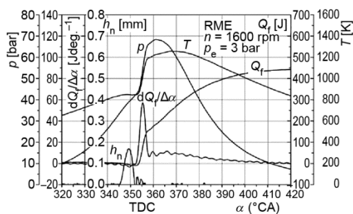
Figure 9. Recorded pressure, p , injector needle lift, h_n , rate of heat release, dQ/d\alpha , cumulative heat released, Q , and mean gas temperature, T ; fuel pure RME
