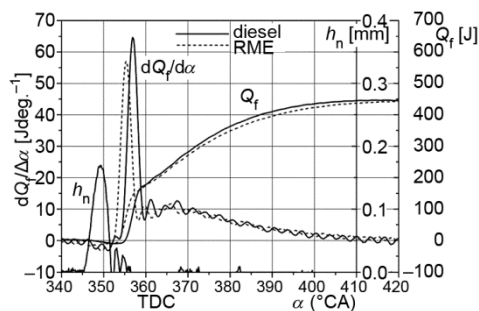
Figure 10. The comparison of combustion dynamics of standard diesel (full line) and pure RME (dashed lines); h_n – the needle lift, dQ/d\alpha – the rate of heat release, Q – the cumulative heat released, p_e = 3 bar, n = 1600 rpm
