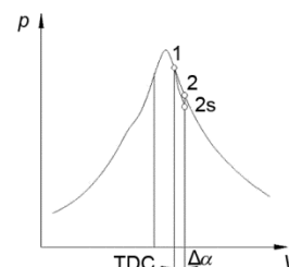
Figure 3. Recorded p - V diagram; gas state change from point 1 to point 2
