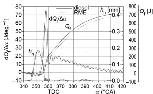
Figure 7. The comparison of combustion dynamics of standard diesel (full line) and pure RME (dashed lines); h_n – the needle lift, dQ/d\alpha – the rate of heat release, Q_f – the cumulative heat released, p_e = 6 bar, n = 1600 rpm
