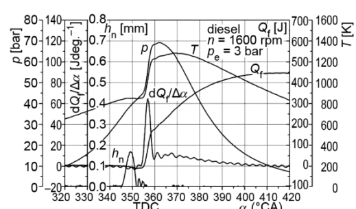
Figure 8. Recorded pressure, p , injector needle lift, h_n , rate of heat release, dQ/d\alpha , cumulative heat released, Q_f , and mean gas temperature, T ; fuel standard diesel
