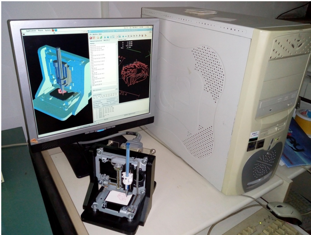
Fig. 12 Machine work environment with PC control system and integrated virtual machine in the background.
