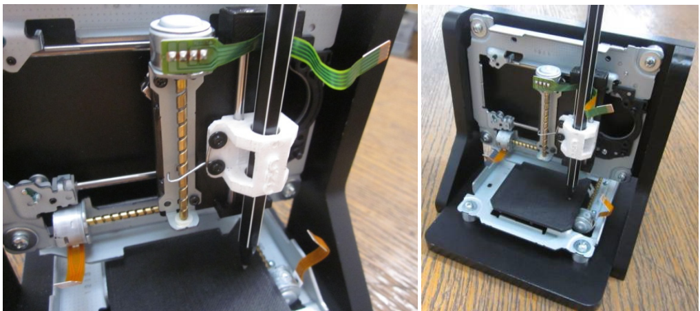
Fig. 6 Fully assembled prototype of the machine
