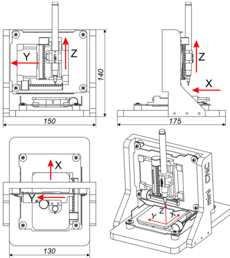
Fig. 3 Drawing views of the complete assembly
