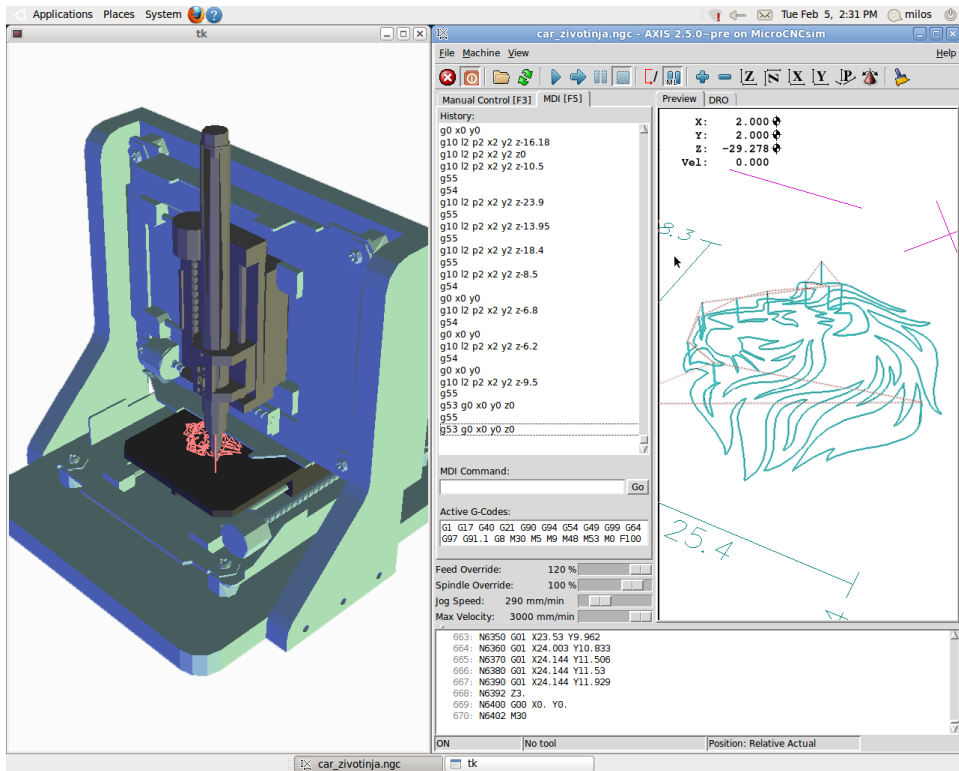
Fig. 9 The Virtual machine integrated with the graphic user interface AXIS
