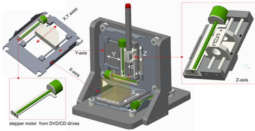
Fig. 2 CAD model of the table 3-axis mini CNC machine tool with basic components
