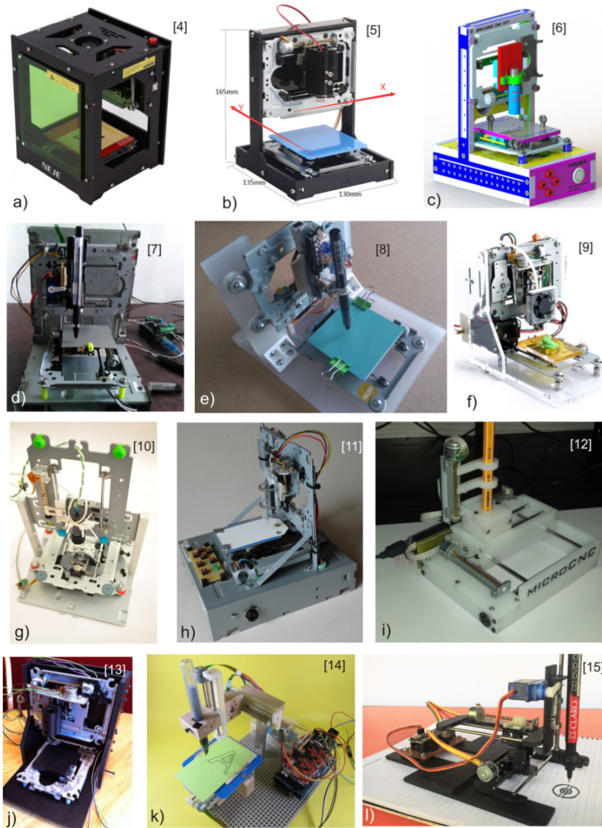
Fig. 1 Mini CNC machine tools based on CD/DVD drive hardware [4-15]
