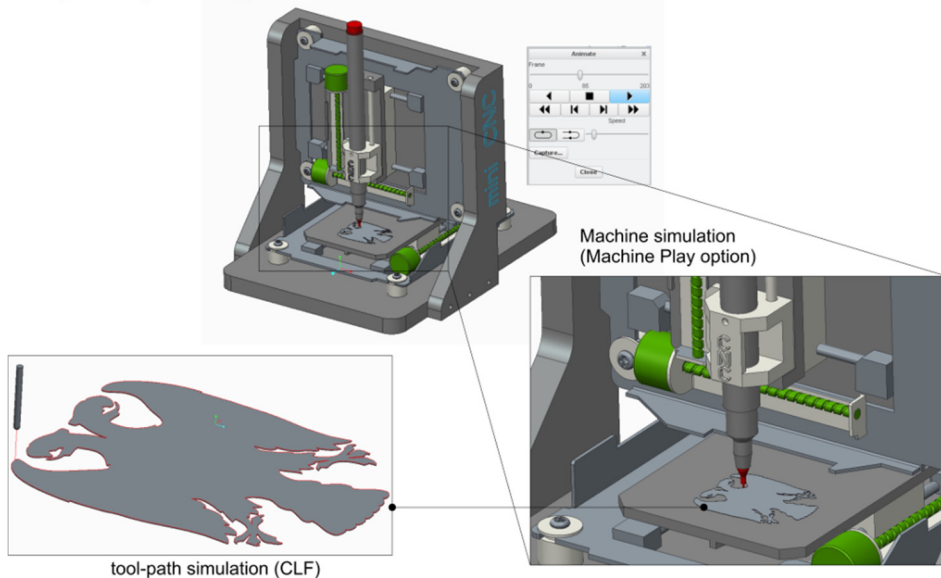
Fig. 4 Example of the simulation within the CAD/CAM environment with active virtual machine executing the given machining program (CLF)
