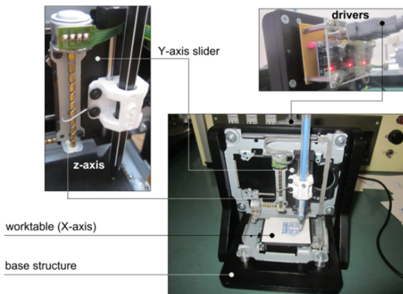
Fig. 10 Fully integrated mechanical and control hardware.
