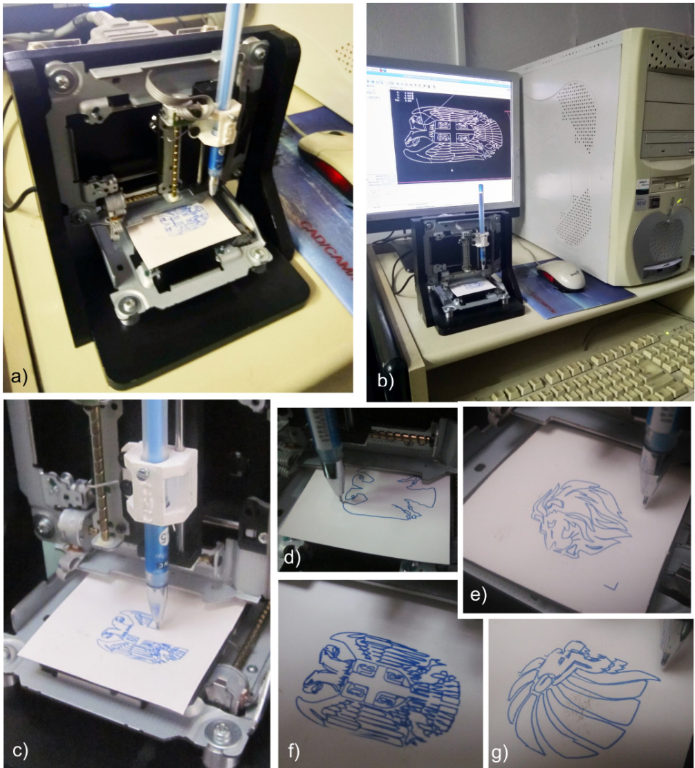
Fig. 11 Machine work environment and results of several trials.
