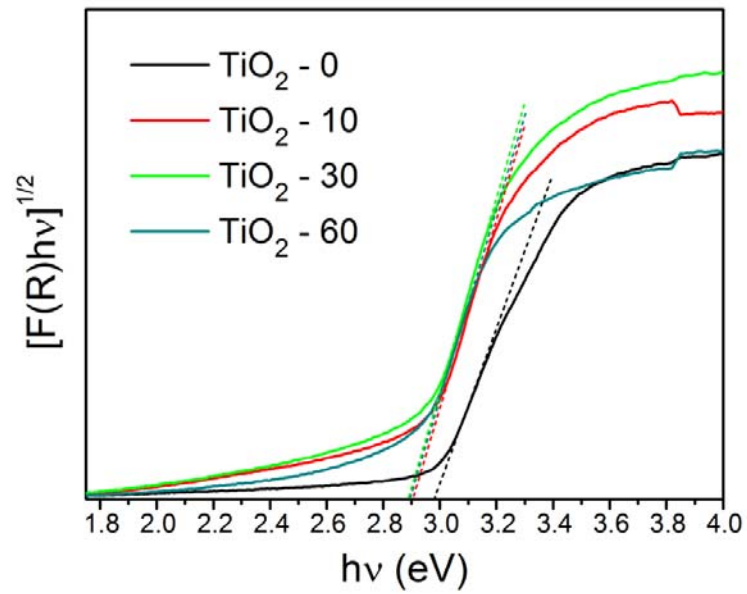
Figure 3. Tauc plot of the transformed Kubelka-Munk function versus photon energy, for non-activated and mechanically activated TiO 2
