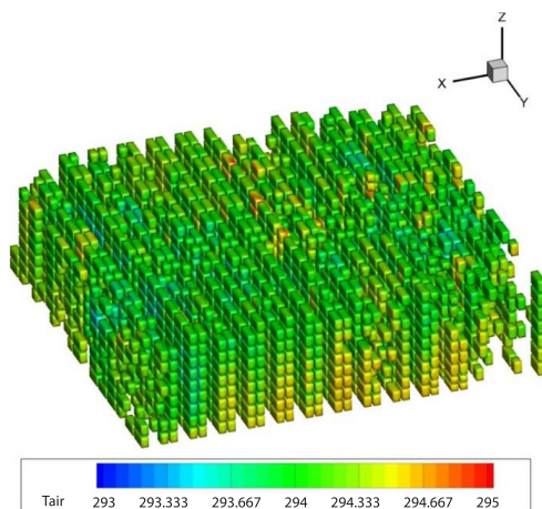
Figure 10. Pallets surface temperature contours, steady-state simulation
