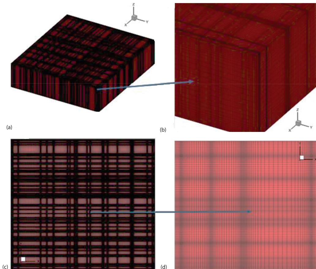
Figure 5. Computational mesh used for numerical simulations; (a) isometric view, (b) isometric view – refinement zone detail, (c) top view, and (d) top view – refinement zone detail (for color image see journal web site)
