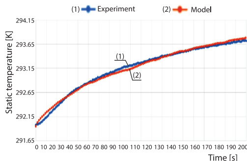
Figure 14. Averaged pallets surface temperature in middle cross-section x = \text{constant} vs. time dependence, comparison between experimental and model results
