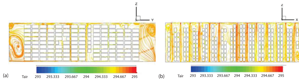
Figure 9. Velocity vectors colored by static temperature; (a) middle x = \text{constant} plane and (b) middle y = \text{constant} plane
