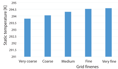
Figure 4. Grid independence study, static temperature vs. grid fineness
