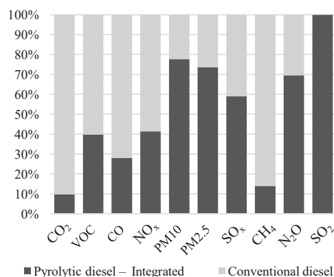
Figure 5. Comparison of pollutant emissions for integrated-internal H 2 pathway and conventional diesel pathway [kg]
