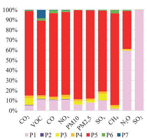
Figure 1. Pollutant emissions during the production of pyrolytic diesel from Miscanthus giganteus [kg] (for color image see journal web site)
