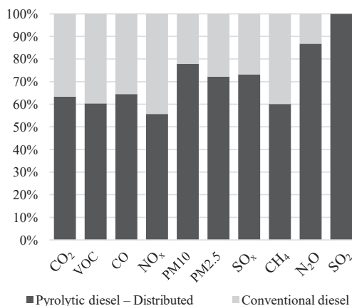
Figure 3. Comparison of pollutant emissions for distributed – external H 2 pathway and conventional diesel pathway [kg]
