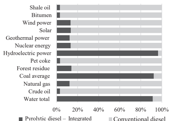
Figure 6. Comparison of resource depletion for integrated-internal H 2 pathway and conventional diesel pathway [MJ]
