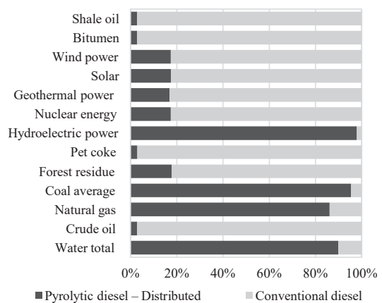
Figure 4. Comparison of resource depletion for external distributed – external H 2 pathway and conventional diesel pathway [MJ]
