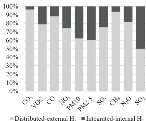
Figure 7. Comparison of pollutant emissions for distributed-external H 2 and integrated-internal H 2 diesel pathway [kg]
