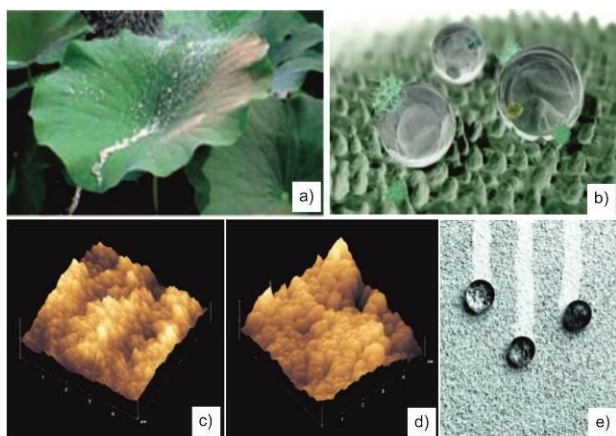
Fig. 3. Lotus effect: (a) lotus leaf, (b) computer graphic of lotus leaf surface, (c) microstructure of lotus leaf surface magnified 7000 times, (d) microstructure on the surface of StoLotusan® magnified 7000 times and (e) self-cleaning effect on paint that makes use of Lotus effect.
