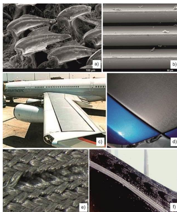
Fig. 6. Riblet effect: (a) microscopic image of shark skin morphology, (b) application in naval industry, (c) application in aircraft industry, (d) application in automotive industry, (e) and (f) application in making swimwear.
