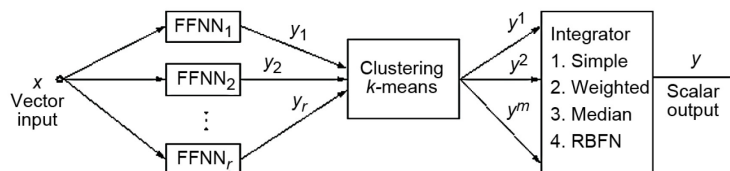
Figure 3. Proposed neural network ensemble
