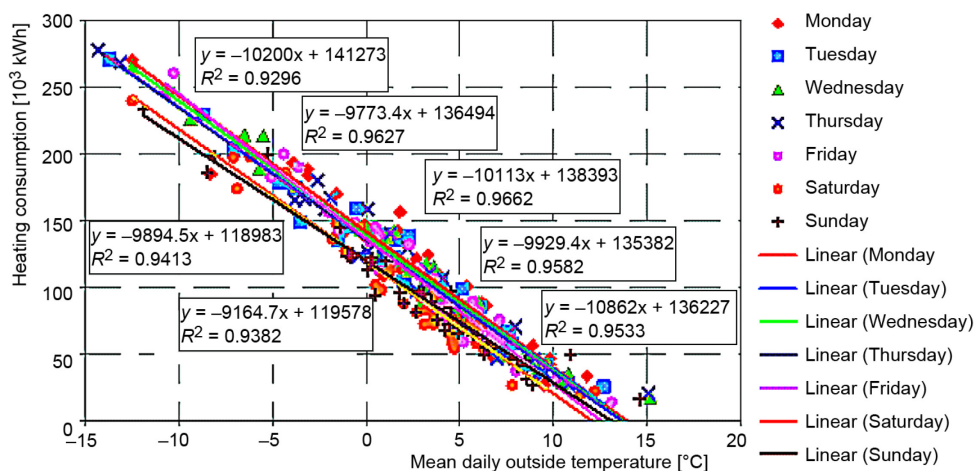
Figure 2. Correlation of the daily heating energy consumption with the mean daily outside temperature for the year 2012 (for color image see journal web-site)
