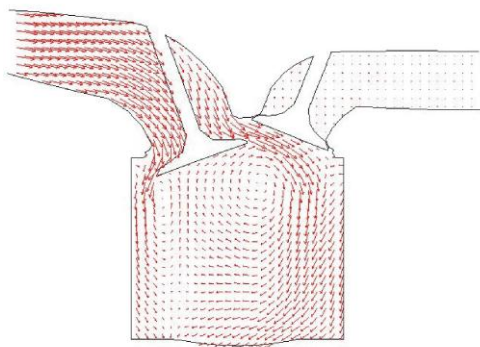
Figure 4. Perspective plot of the combustion chamber and valve/port geometry layout (squish area = 62%, cylindrical bowl) k-\varepsilon model
