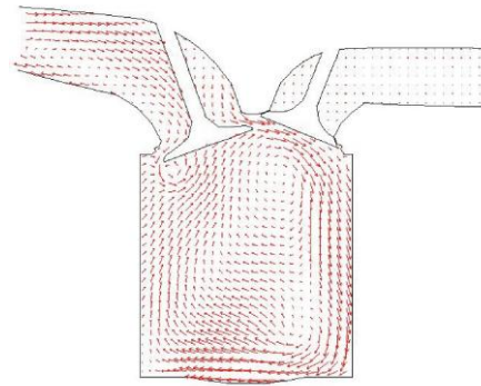
Figure 5. Fluid flow pattern in x-z plane, y = 2.1 cm, at 170^\circ aTDC, k-\varepsilon model
