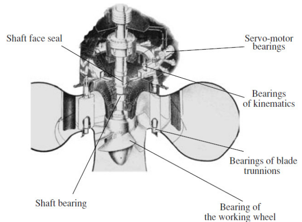
Figure 5. Sliding friction unit of a hydraulic turbine
