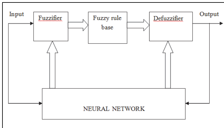
Fig. 2 A fuzzy system whose membership functions is adjusted by a neural network
