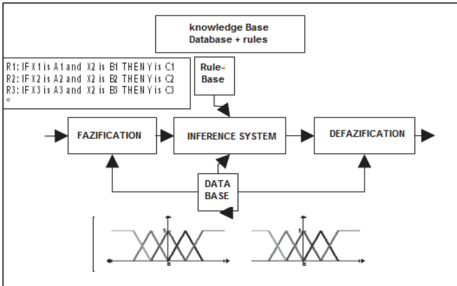
Fig. 1 The generic structure of the fuzzy system
