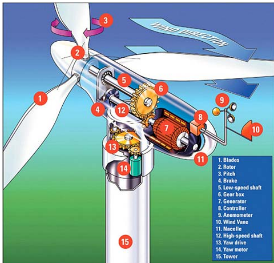
Figure 4. Wind generator
