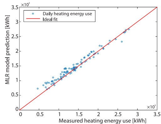
Figure 2. The MLR model vs. measured data for the test period
