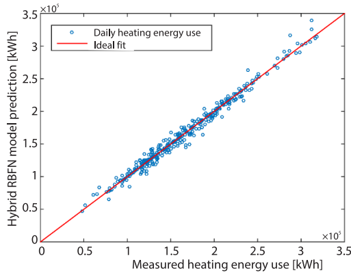
Figure 7. Hybrid RBFN model vs. measured data for the training period
