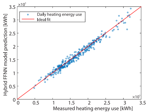
Figure 3. Hybrid FFNN model vs. measured data for the training period
