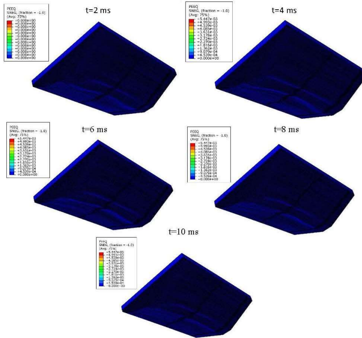
Figure 8. Evolution of equivalent plastic deformation (PEEQ) for 5 different moments after detonation for the case when \alpha=155^\circ and \beta=120^\circ
