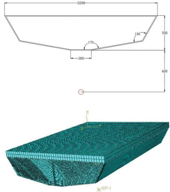
Figure 2. V-hull geometry and finite element mesh for the numerical model and the FEM vehicle model and the position of the explosive charge when \alpha=170^\circ and \beta=130^\circ
