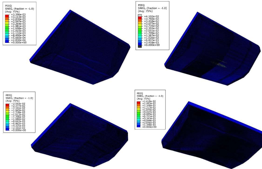
Figure 3. Equivalent plastic deformation (PEEQ) for 4 different cases at 10 ms after detonation
