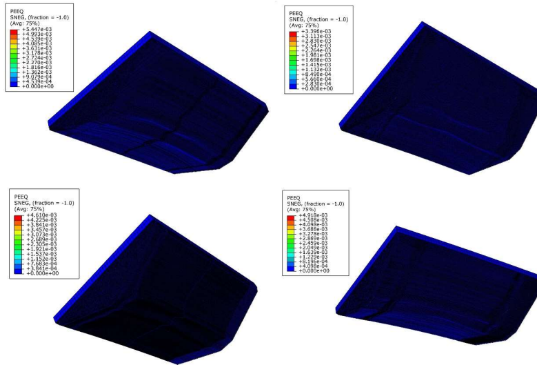
Figure 6. Equivalent plastic strain distribution (PEEQ) for 4 different cases at 10 ms after detonation
