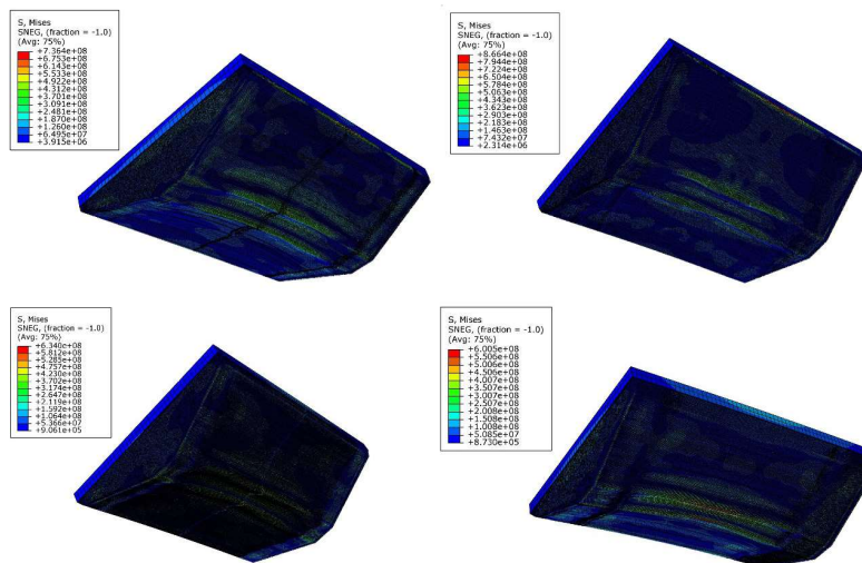
Figure 7. Equivalent of von Mises stress distribution in loaded structure for 4 different cases at 10 ms after detonation
