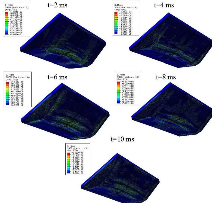
Figure 9. Evolution of von Mises stress in loaded structure at 5 different moments after detonation for the case when \alpha=155^\circ and \beta=120^\circ
