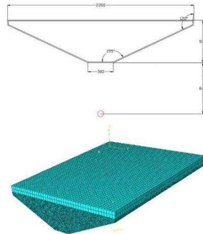
Figure 5. V hull geometry and finite element mesh for the numerical model and the FEM vehicle model and the position of the explosive charge when \alpha=155^\circ and \beta=120^\circ
