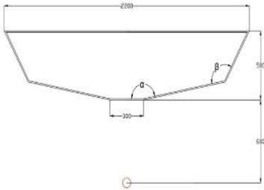
Figure 1. Geometry of the V-shaped hull used in numerical model
