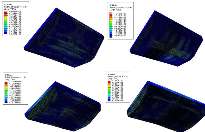
Figure 4. Von Mises stress in loaded structure for 4 different cases at 10 ms after detonation
