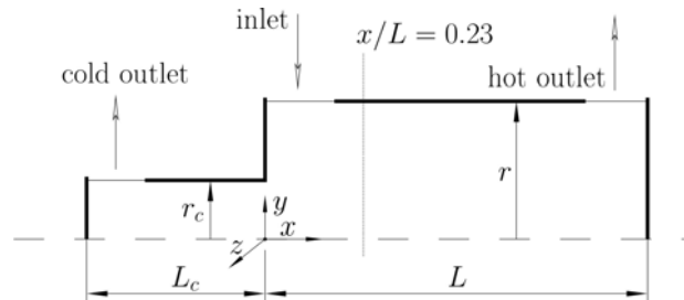
Figure 1. Geometry of the vortex tube [6]
