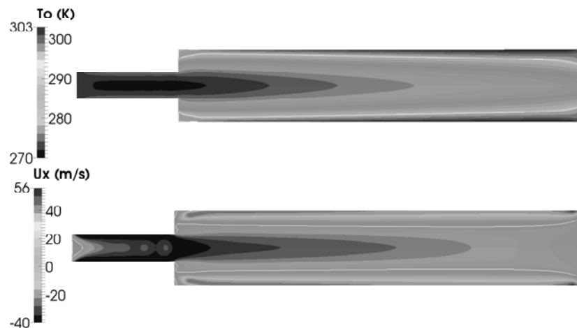
Figure 6. Total temperature and axial velocity contours – white lines designate contour T_0 = 294\text{K} (value of inlet total temperature) and U_x = 0\text{ms}^{-1} ; solver rhoCentralTurbFoam, k-\omega SST model (for color image see journal website)
