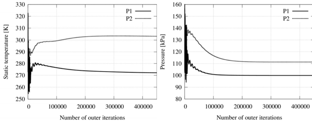
Figure 3. Changes of temperature and pressure during iteration procedure. Mesh M2, k-\varepsilon turbulence model, solver steadyCompressibleTEFoam. Point coordinates: P1(0.01,0.001,0), P2(0.3,0.001,0)
