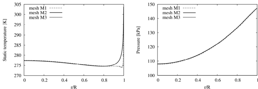
Figure 2. Mesh independence test results in cross section x/L = 0.23 with the use of the k-\epsilon model and steadyCompressibleTEFoam solver
