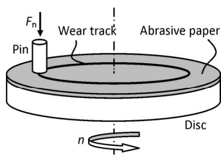
Fig. 2. Schematic diagram of abrasion testing.
