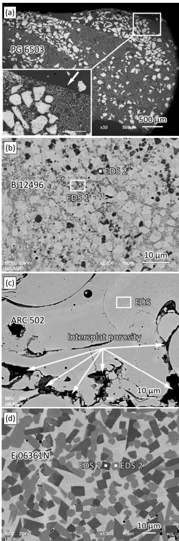
Fig. 3. Microstructure properties of tested coatings.
