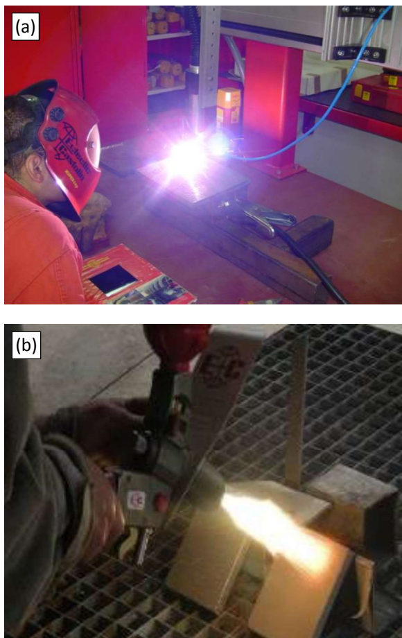
Fig. 1. Experimental setup for: (a) PTA deposition and (b) FS deposition.
