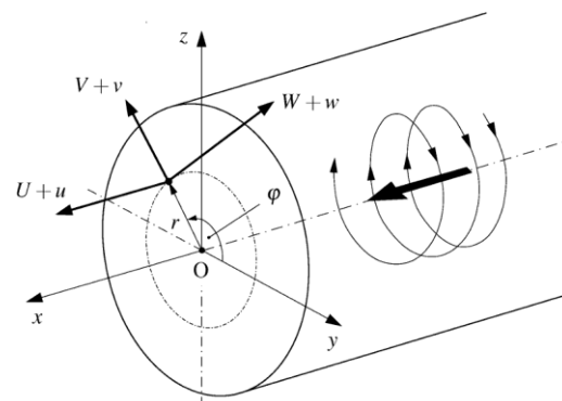
Figure 1. Coordinate system and velocities in turbulent swirling flow in the pipe.
