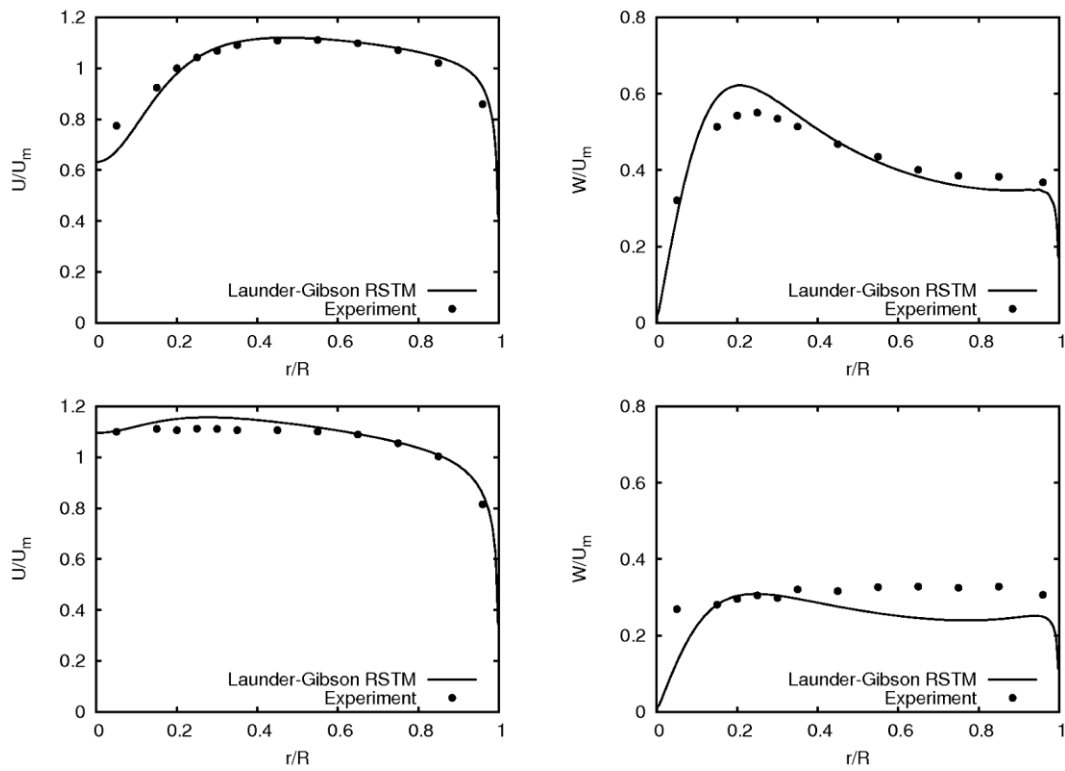
Figure 5. Profiles of mean velocities U and W for \theta_p=0.229 . First line: measuring section x/R = 33 , second line: measuring section x/R = 90 .
