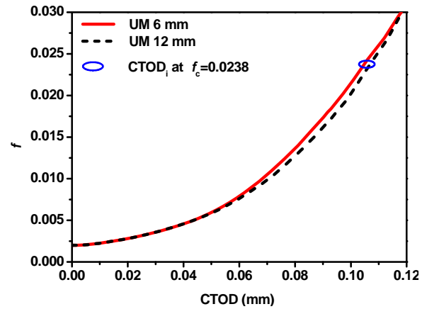
Figure 6. Void volume fraction f vs. crack tip opening displacement CTOD by GTN model for C(T) specimen with two different widths of UM weld metal.
