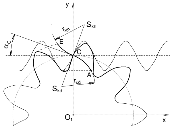
Figure 2. Shape of the convex-concave gear-tooth profile
