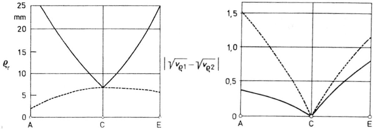
Figure 4. Mean curvature radius and the difference of square roots of the tangential speeds along the path of contact for convex-concave and involute gear-teeth
