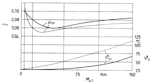
Figure 6. Measured bulk temperature on test gears for initial oil temperature T_{ol} = 20^\circ\text{C}
