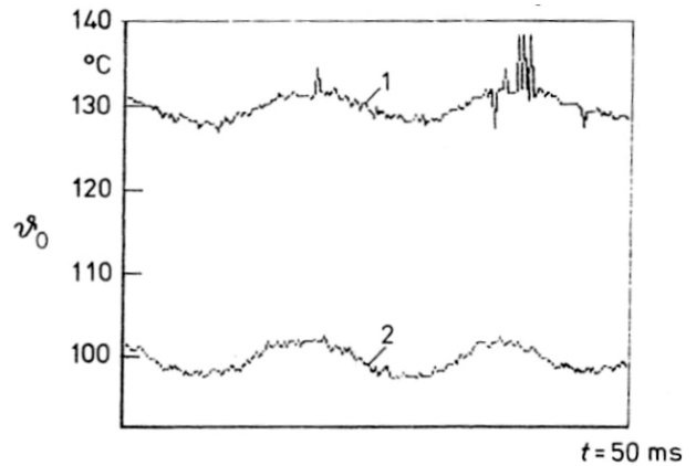
Figure 5. Oil temperature for convex-concave (2) and involute (1) teeth form measured in the FZG gear-rig machine (without additional oil heating)
