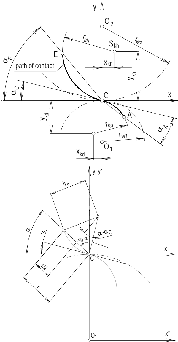
Figure 1. Definition of convex-concave cylindrical gear flanks
